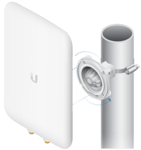
Pole-Mount Installation
